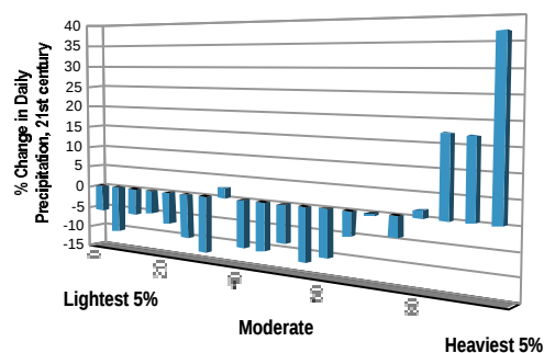
Hadley Model
