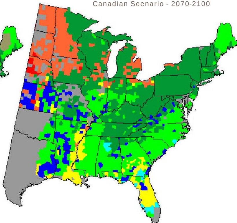
Canadian Scenario - 2070-2100
