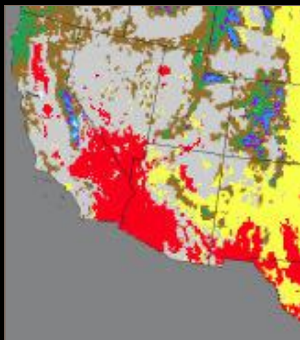
Current Ecosystems
