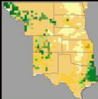
Soil C (g/sq m)
