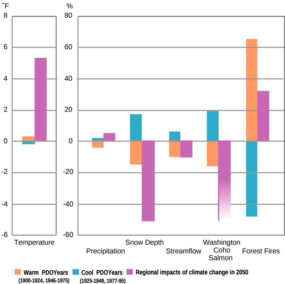
Regional Impacts: Climate Change projected for 2050 vs observed 20th century variability
