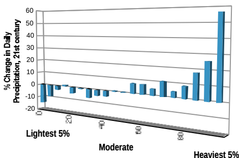
Canadian Model
