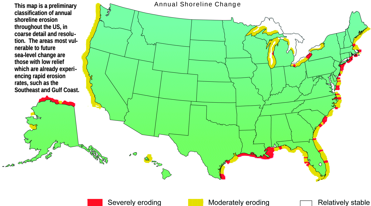
Annual Shoreline Change
