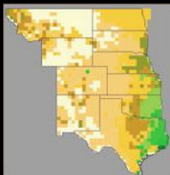
NPP (g/sq m)
