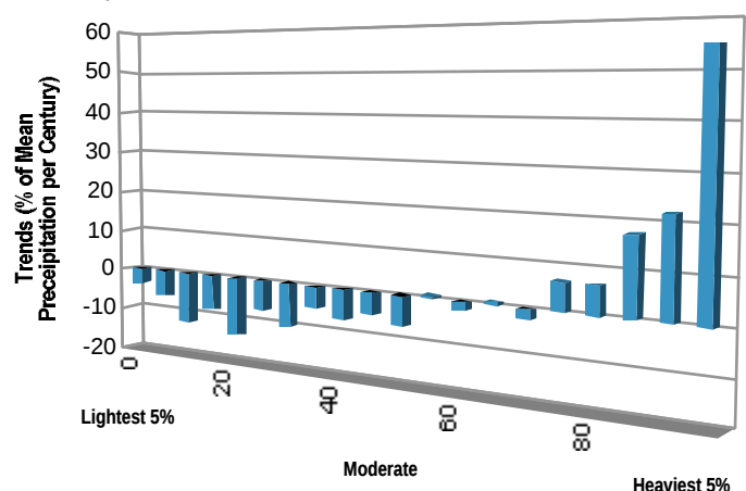
Hadley Model
