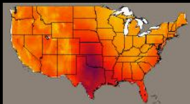
Hadley Model
